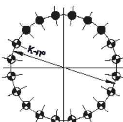
DN 20" - 24"
